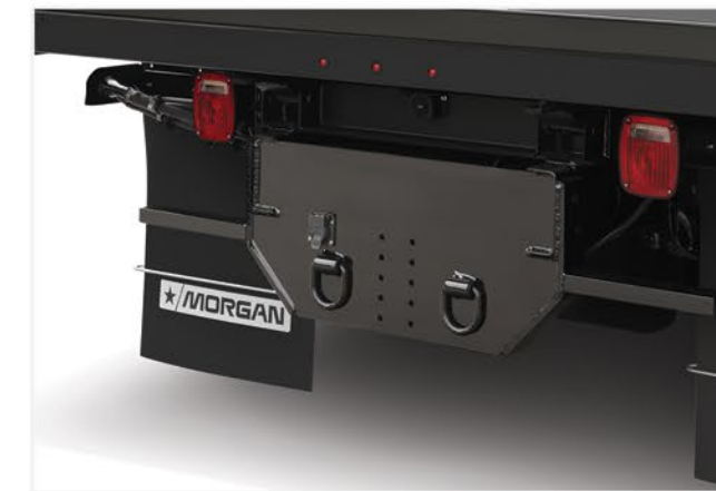
Chassis-mounted features such as the underbody bumper, hitch plate, mudflap mounts, anti-sail braces, and fuel and DEF-fill ports, minimize wear and tear on components and support greater longevity and performance.
